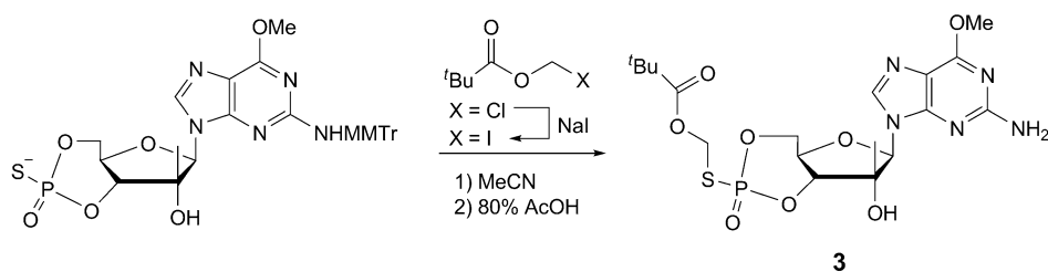
Scheme 4. Preparation of the of 2'-C, O 6 -Dimethylguanosine 3',5'-Cyclic (S-(Pivaloyloxy)methyl Phosphorothioate)
