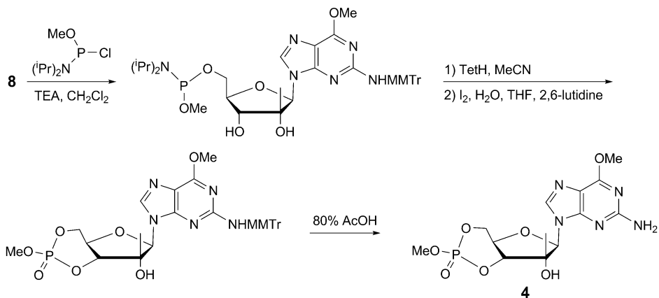
Scheme 5. Preparation of the of 2'-C, O 6 -Dimethylguanosine 3',5'-Cyclic (Methyl Phosphate)
