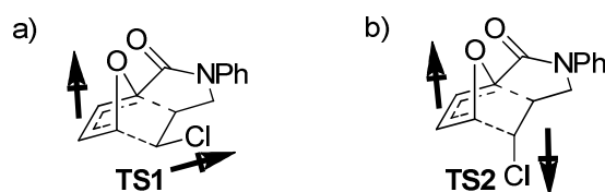
Scheme 1 a) Unfavorable and b) favorable dipolar interactions
