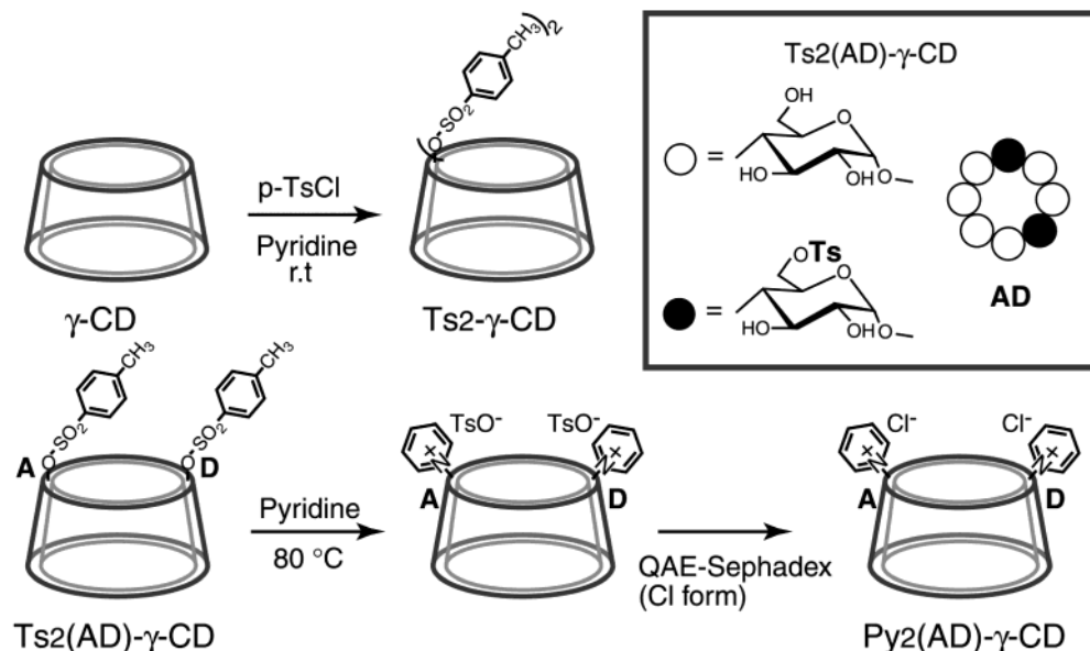
Scheme 1. Synthesis of 6A,6D-Bispyridinio- \gamma -CD ( Py2(AD)- \gamma -CD )
