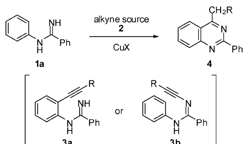
Scheme 1. Direct Synthesis of Quinazoline through Copper-Catalyzed Alkynylation and Cyclization
