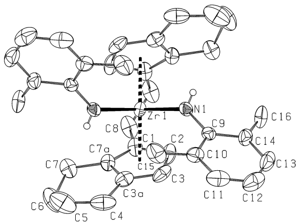
Fig. 1. PLATON-drawing of rac - 3a . Hydrogen atoms (except NH) are omitted for clarity. Thermal ellipsoids are drawn at 30% probability level. Selected bond lengths (pm) and angles (°): Zr(1)–C(1) 253.2(4), Zr(1)–C(2) 246.0(5), Zr(1)–C(3) 252.4(3), Zr(1)–C(3a) 264.0(4), Zr(1)–C(7a) 262.8(4), Zr(1)–N(1) 213.7(3), C(1)–C(8) 150.7(5), C(8)–C(8') 153.0(6), N(1)–C(9) 141.9(5), C(9)–C(10) 140.2(6), C(9)–C(14) 141.2(5), C(10)–C(15) 151.3(6), C(14)–C(16) 150.4(6), N(1)–Zr(1)–N(1) 105.9(1), Zr(1)–N(1)–C(9) 138.9(2), N(1)–C(9)–C(10) 121.1(3), N(1)–C(9)–C(14) 121.5(4), C(9)–C(10)–C(15) 122.7(4), C(9)–C(14)–C(16) 119.9(4), C g –Zr(1)–C g 123.7, (C g defines the centers of gravity of the five-membered rings of the corresponding tetrahydroindenyl systems).
