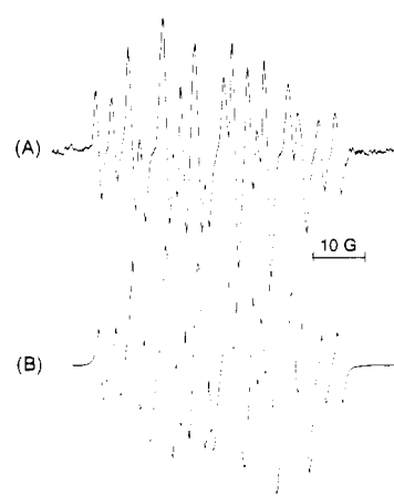
Figure 3. (A) EPR spectrum from system containing i -AmONO (21 mmol L -1 ), 3d (10 mmol L -1 ), and DMPO (170 mmol L -1 ) in deaerated benzene. Experimental settings: modulation amplitude 0.27 G, gain 4 \times 10^5 , others as in Figure 1A. (B) Simulated spectrum (coupling constants in Table III).
