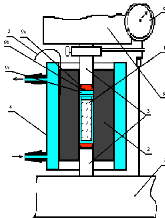
Figure 2. Reaction block for performing chemical reactions at high pressures: 1- Teflon ampoule for reaction mixture; 2- High-pressure block of constructional steel with hardness HRC 40-42; 3- Steel pistons with hardness HRC 58-60; 4- thermostatic jacket; 5- thermocouple; 6- Press plunger; 7- Press frame support; 8- Micrometer. Reaction volume compression comprise from: an anti-extrusion steel ring - 9a, a copper disk - 9b, a Teflon disk - 9c.
