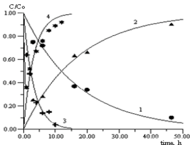
Figure 3. Kinetic curves of the diaziridine 1a formation from N -chloroethylamine 3a at high pressure. Curves 1 and 3 correspond to consumption of N -chloroethylamine 3a . Curves 2 and 4 correspond to accumulation of diaziridine 1a . Curves 1 and 2 were recorded at 300 MPa. Curves 3 and 4 were recorded at 500 MPa.
