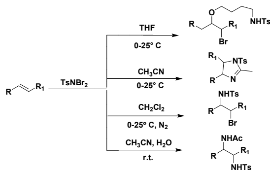
Scheme 1: Aminofunctionalization of olefins using TsNBr 2
