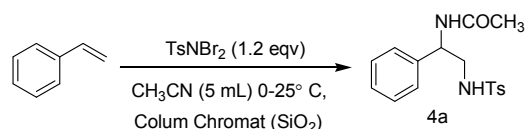
Scheme 2: Formation N -acetyl, N' -tosyl diamine from styrene
