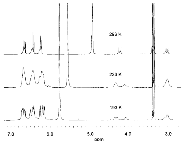
Figure 4. Variable-temperature ^1\text{H} NMR spectra of \text{Li}_4[(\text{I})_3\text{Ti}_2] (in [\text{D}_4]\text{methanol} ).
