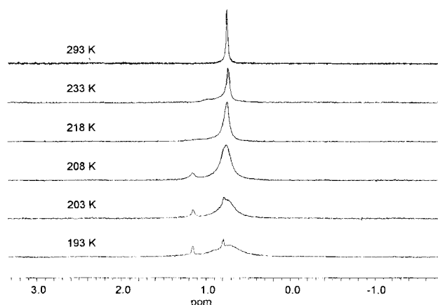
Figure 5. Variable-temperature ^6\text{Li} NMR spectra of ^6\text{Li}_4[(\text{I})_3\text{Ti}_2] (in [\text{D}_4]\text{methanol} ).
