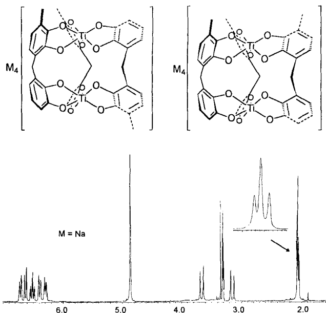
Figure 8. ^1\text{H} NMR spectrum of \text{Na}_4[(3)_3\text{Ti}_2] in [\text{D}_4]\text{methanol} . The signals of the methyl groups at \delta = 2.0 – 2.1 indicate the presence of a 4:1 mixture of the unsymmetrical (left) and the C_3 -symmetrical isomer (right).
