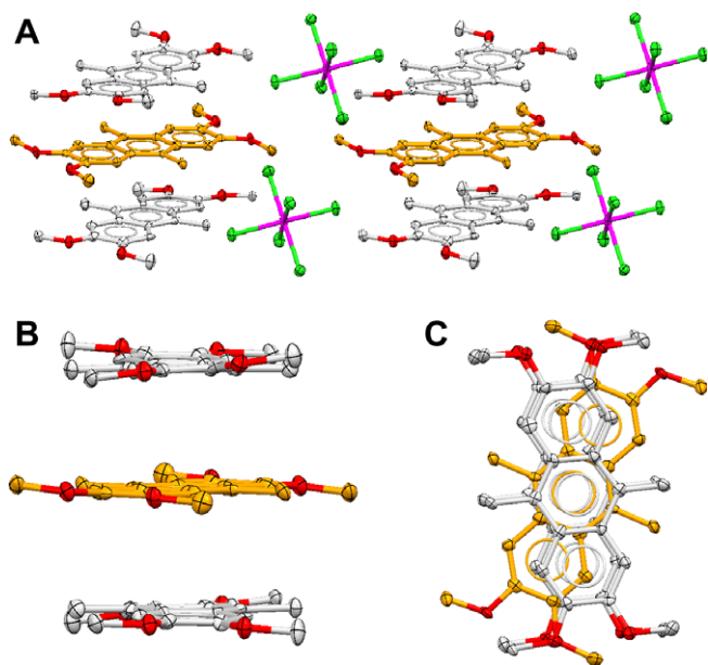
Figure 4. Crystal structure of the tetramethoxydimethylantracene cation radical with the packing diagram (A) showing that it crystallizes as a centrosymmetric homotrimer (B and C) with a pair of cationic charges [(SbCl 6 − ) 2 ]. The thermal ellipsoids are shown in 50% probability and the hydrogens and solvent molecules (CH 2 Cl 2 ) are omitted for the sake of clarity.
