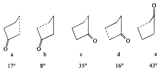
Scheme 9. Envelope Conformations for Cyclopentanone, Showing the Possible Relations of the Carbonyl to the Bond That Would Cleave in a Retro-aldol Reaction of 3-Hydroxy-3-methylcyclopentanone a
