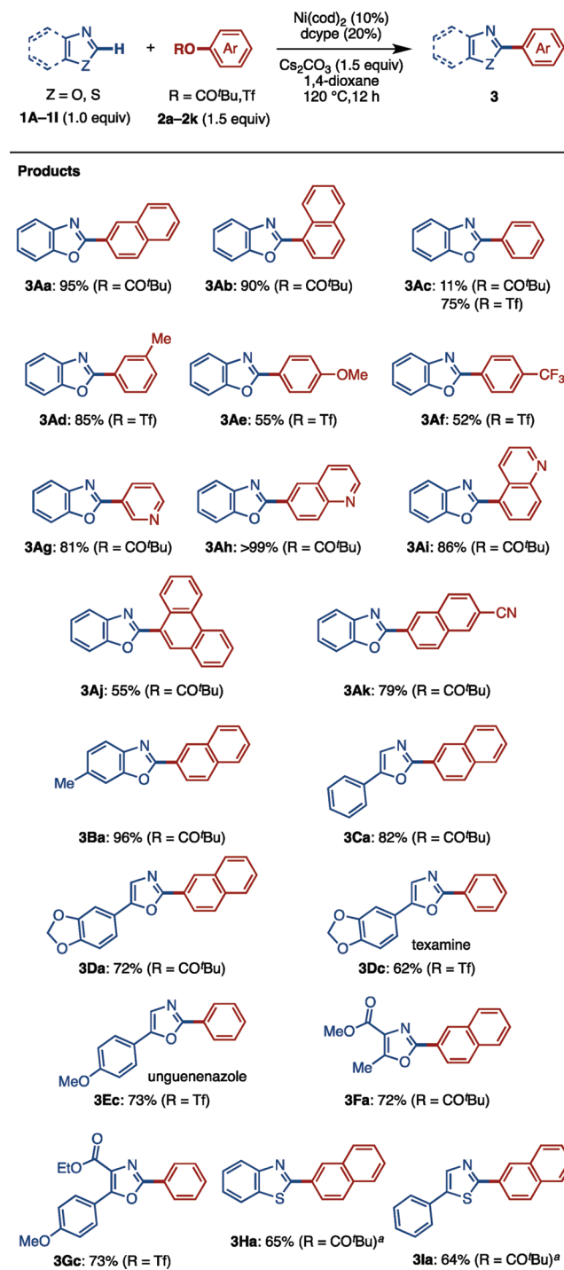
Scheme 4. C–H/C–O Biaryl Coupling Catalyzed by the Ni/dcype System
