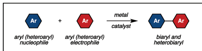
Scheme 1. Recent Directions in Catalyzed Biaryl Coupling
