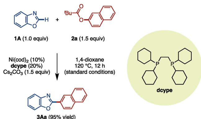
Scheme 2. Discovery of the Ni(cod) 2 /dcype Catalyst for C–H/C–O Biaryl Coupling
