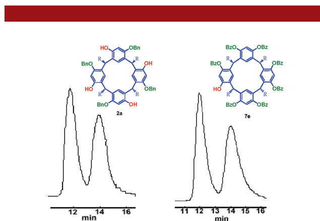
Figure 3. HPLC enantioresolution of compounds 2a and 7e (left and right, respectively) at 98/2 (v/v) of n -hexane/2-propanol. Flow rate = 0.6 and 0.8 mL/min, respectively.
