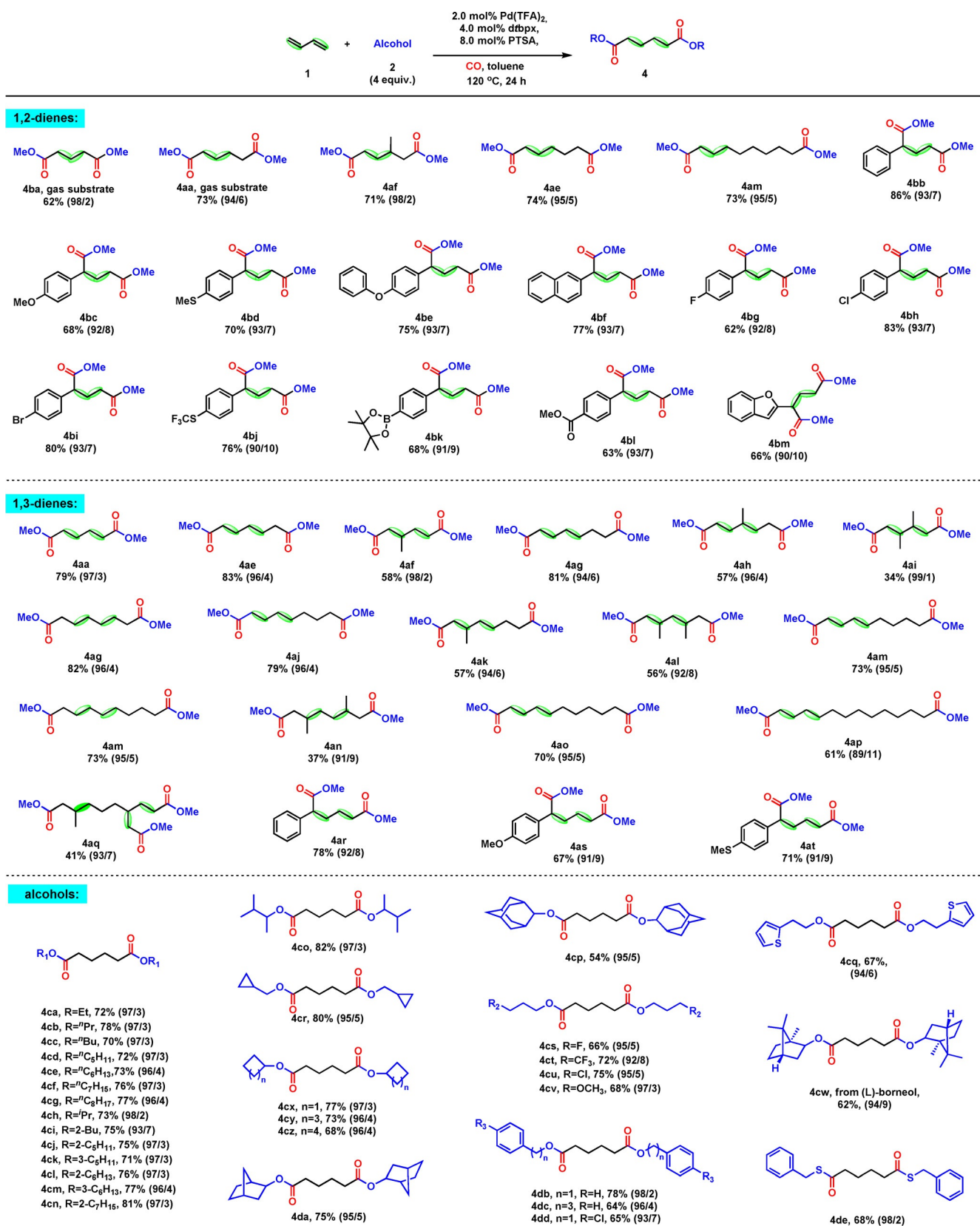
Figure 4. Substrate scope for various dienes and alcohols. Yields are reported as isolated yields; the selectivity is the ratio of the linear diester to branched diesters, which is determined by GC analysis.
