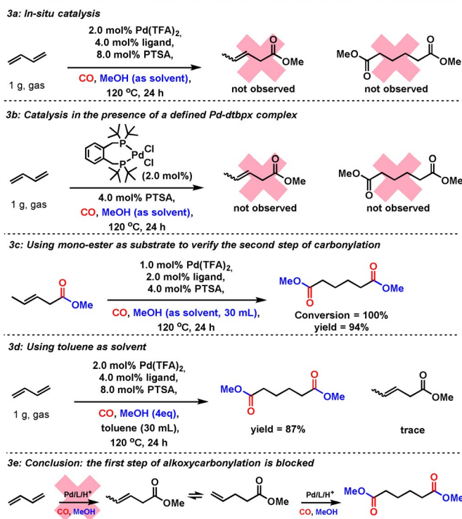
Scheme 3. Selected control experiments.
