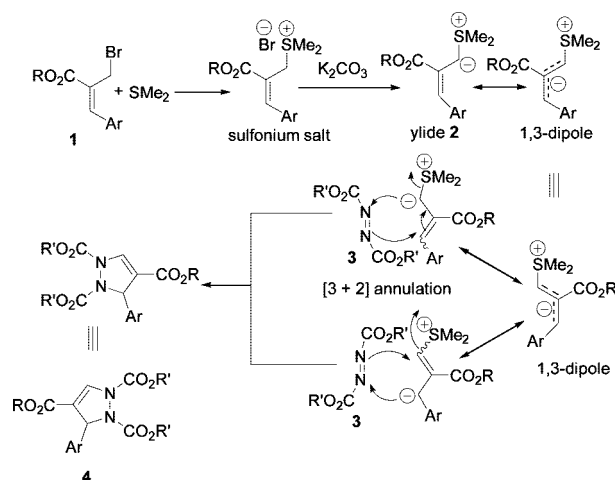
Scheme 3. Plausible Mechanism
