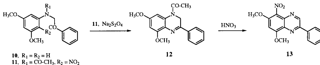
Scheme 2: Alternative Synthesis of the Lead Compound
