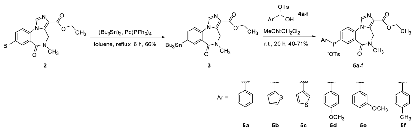
Scheme 1 Sxynthesis of various diaryliodonium tosylate precursors.
