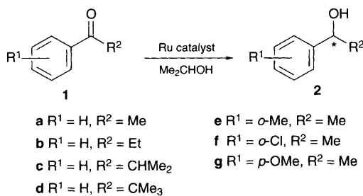
Scheme 1 Reagents and conditions: 0.25 mol % [\{\text{RuCl}_2(\eta^6\text{-arene})\}_2] ; 1 mol % β-amino alcohol; 2.5 mol % KOH. [ketone] = 0.1 mol dm –3 in propan-2-ol, 28 °C.
