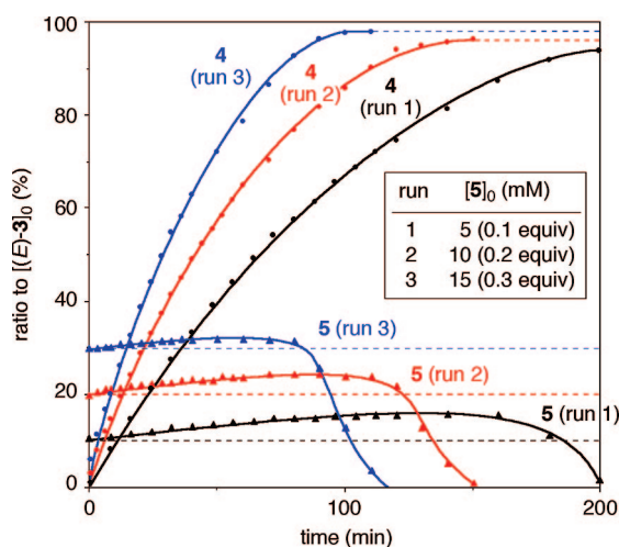
Figure 2. Time course of the reaction of ( E )-3 (50 mM) with ( E )-1 (1.0 M) in C_6D_6/CD_2Cl_2 (5:1 v/v) at 50 °C in the presence of isolated 5.
