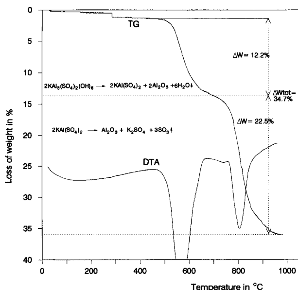
Fig. 3. Thermal curves (TG/DTA) of the alunite used for the mixtures.
