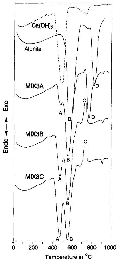
Fig. 6. Thermal curves (DTA) of the alunitite/ \text{Ca(OH)}_2 mixtures. Stoichiometric ratio alunitite/ \text{Ca(OH)}_2 : MIXA = 0.5, MIXB = 1.0, MIXC = 1.5. The curves of pure \text{Ca(OH)}_2 and alunitite are also reported.
