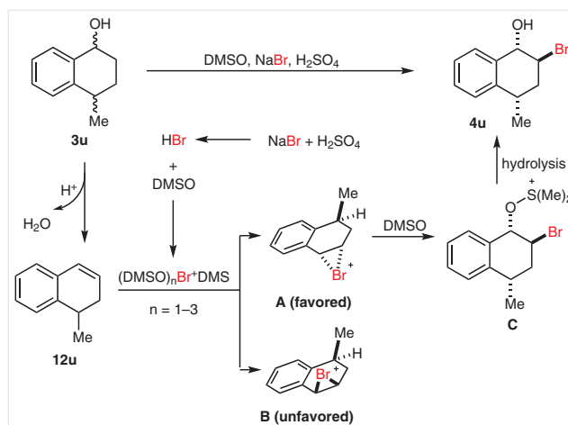
Scheme 8 Proposed mechanism
