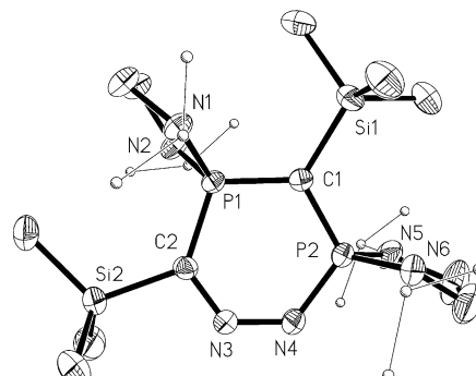
Figure 2. Structure of six-membered heterocycle 8 (thermal ellipsoids drawn at 50% probability for non-hydrogen atoms; hydrogen atoms omitted for clarity).
