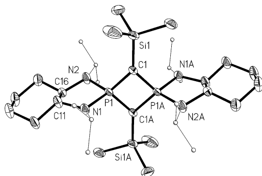
Figure 1. Structure of 1,3-diphosphete 4 (thermal ellipsoids drawn at 50% probability for non-hydrogen atoms; hydrogen atoms omitted for clarity).
