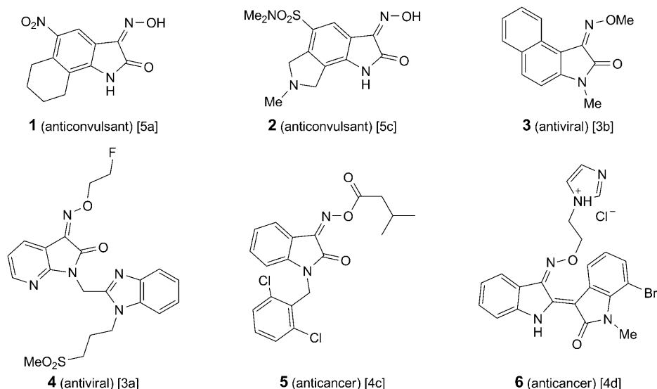
Figure. Structures of several isatin oximes and O-alkyloximes exhibiting biological activities
