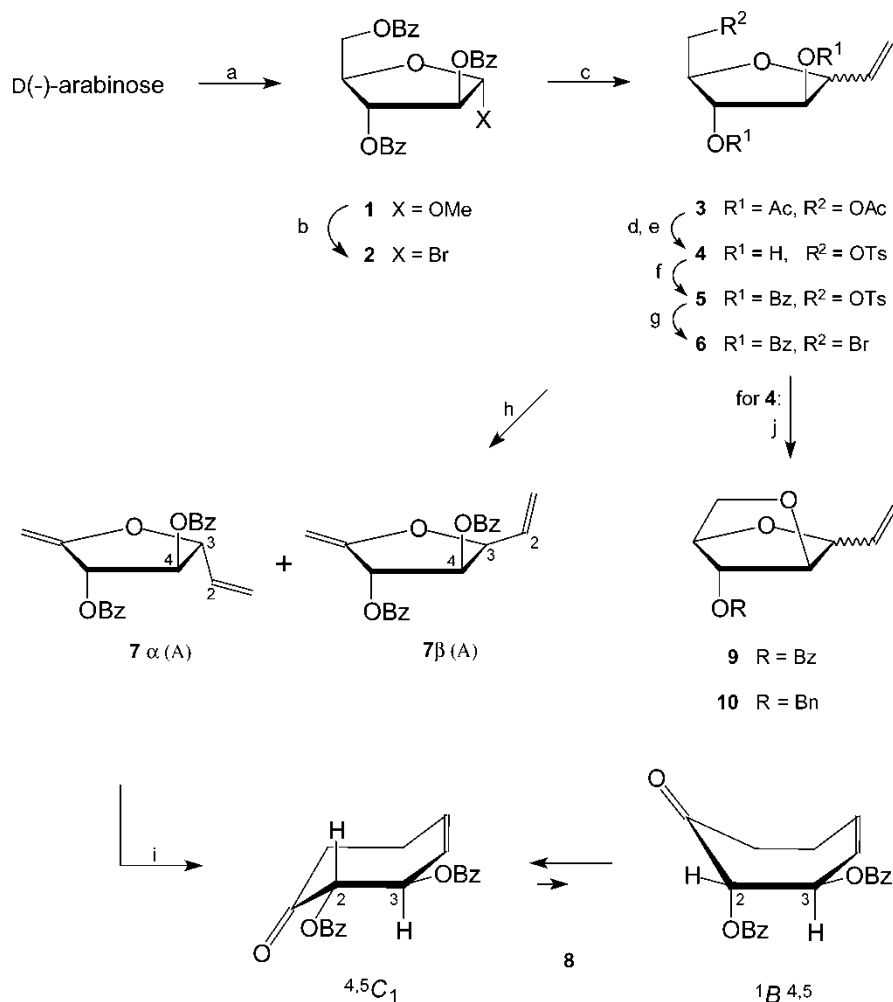
Scheme 1: Claisen rearrangement of a D(-)-arabinose derived furanose precursor a) AcCl, MeOH, then BzCl, py, 79%; b) HBr/HOAc, in situ; c) CH 2 =CHMgBr, THF, then Ac 2 O, py, 66%; d) NaOMe, MeOH, 100%; e) TsCl, py; f) BzCl, DMAP, py, 61% (two steps); g) NaBr, DMF, 70° C, 100%; h) AgF, py, 52%; i) decane/toluene 6:1, microwave, 180° C, 20 min, 54%; j) "basic conditions" (TsCl, py; NaH, BnBr, DMF, respectively).
