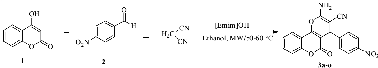
Scheme-I: Synthetic path of 3,4-Dihydropyrano[ c ]chromene derivatives
