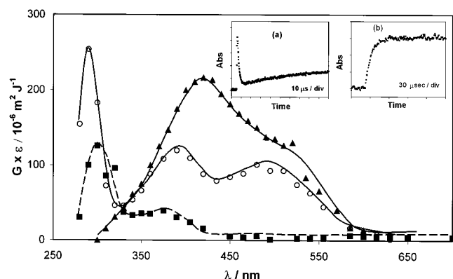
Figure 3. Transient absorption spectra obtained in \text{N}_2\text{O} saturated aqueous solutions of DHMP ( 1 \times 10^{-3} \text{ mol dm}^{-3} ) at 1 \mu\text{s} after the pulse at pH 6 ( \blacktriangle ) and at 2 \mu\text{s} ( \circ ) and 90 \mu\text{s} ( \blacklozenge ) after the pulse at pH 10.5 (dose per pulse = 15 Gy). Inset: (a) intermediate trace obtained at 290 nm at pH 10.4. (b) The \text{TMPD}^{+\bullet} build-up at 565 nm obtained with DHMP ( 2 \times 10^{-3} \text{ mol dm}^{-3} ) in the presence of TMPD at pH 10.4 ( 5 \times 10^{-5} \text{ mol dm}^{-3} ) (dose per pulse = 5 Gy).
