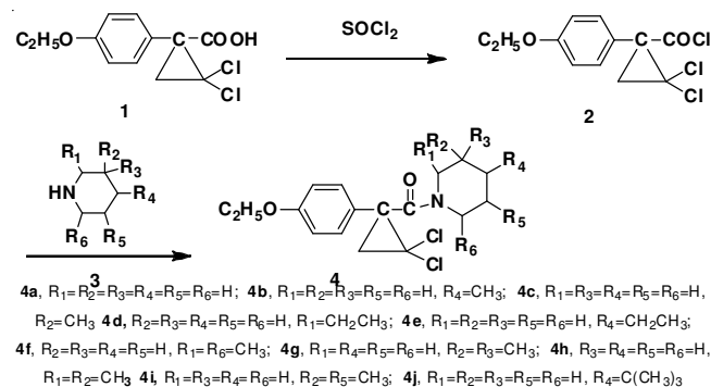
Scheme-I: Synthetic route of title compounds
