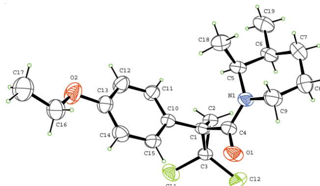
Fig. 2. Molecular structure of 4h
