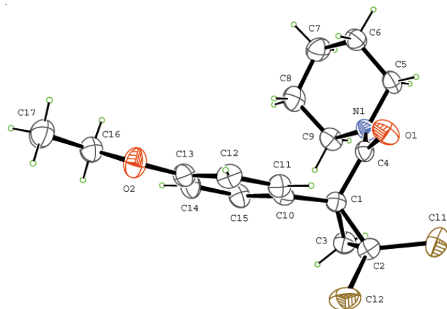
Fig. 1. Molecular structure of 4a
