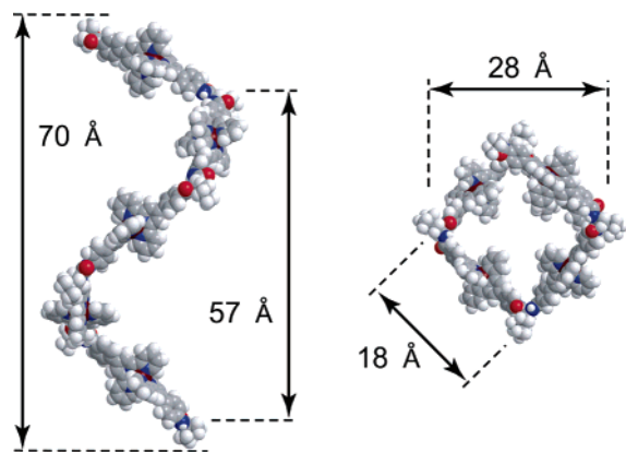
Figure 3. Solution structure of tetramer 4 based on the ^1\text{H} NMR analysis; side (left) and top (right) views.
