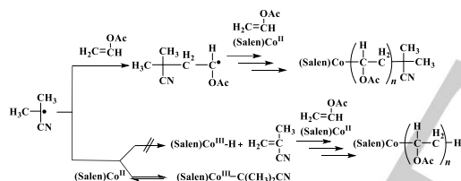
Figure 2. Plausible pathway for PVAc with cyanoisopropyl chain end group. Reactions of the cyanoisopropyl radical with (Salen)Co II and VAc.
