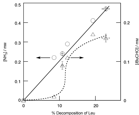
Figure 4. Yields of ammonia (○) and isovaleraldehyde ( i BuCHO, △) as a function of the photodecomposition of neutral Leu (6.63–6.95 mM) upon irradiation by l -CPL of varying doses (100–860 mA h) at 21 K.
