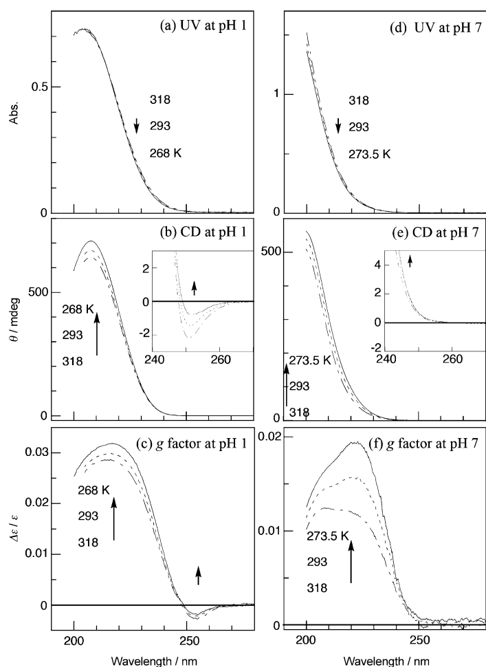
Figure 1. UV (top), CD (middle), and anisotropy spectra (bottom) of acidic (left) and neutral (right) aqueous solutions of L-Leu (10.6 mM for the acidic solution and 106 mM for the neutral solution) at 318–268 K. The UV and CD spectra at 318 and 293 K are corrected for the volume changes caused by temperature variation, whereas the anisotropy factor is inherently free from the errors arising from volume change as g = \Delta\epsilon/\epsilon .
