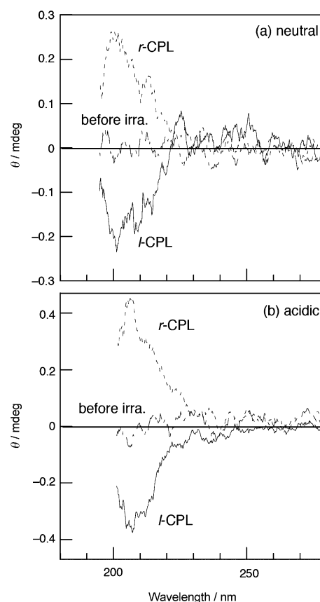
Figure 2. CD spectra of rac -Leu solutions recorded at 296 K before and after CPL irradiation at 215 nm in an ice matrix at 21 K. (a) Neutral samples ( [rac\text{-Leu}] = 7.0 mM, \text{pH}_{298\text{K}} = 7 ), in which the conversions upon irradiation of l - and r -CPL (dose: 860 mA h) were 21 and 17%, respectively. (b) Acidic samples ( [rac\text{-Leu}] = 30.5 mM, \text{pH}_{298\text{K}} = 1 ), in which the conversions upon irradiation of l - and r -CPL (dose: 400 mA h) were 6 and 7%, respectively.
