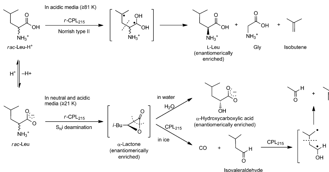
Scheme 1. Photochemical reactions of rac -Leu in acidic and neutral aqueous solutions and ice matrices.
