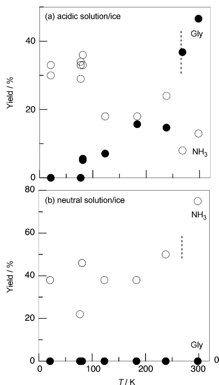
Figure 3. Chemical yields of ammonia (○) and Gly (●) obtained upon irradiation of (a) acidic and (b) neutral rac -Leu samples in aqueous solutions at 268–298 K and in ice matrices at 21–238 K. The vertical broken line indicates the freezing point of each solution.
