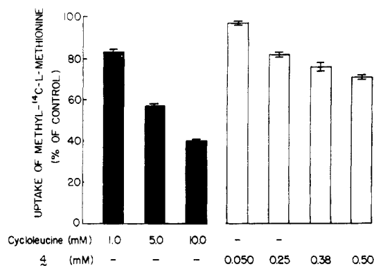
Figure 2. Inhibition of [methyl- ^{14}C ]-L-methionine uptake into Ehrlich ascites cells by 2-aminoadamantane-2-carboxylic acid (4) compared against cycloleucine (1c). Details as in Figure 1.
