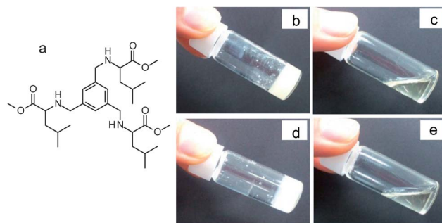
Fig. 4 (a) Molecular structure of compound A . (b–e) Photographs of ionic liquids, containing (b and d) gelator 4 and (c and e) compound A . Solvents were (b and c) [BuMeIm][TFSA] and (d and e) [BuMeIm][CF 3 SO 3 ]. The concentrations of gelator 4 and compound A were 2.0 wt%.
