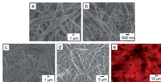
Fig. 1 FE-SEM images of (a and b) ionogels and (c and d) organogels, formed in the respective solvents: [BuMeIm][TfSA], [BuMeIm][CF 3 SO 3 ], ethanol, and acetonitrile. (e) CLSM image of the ionogel stained by 30 \mu M rhodamine B (solvent: [BuMeIm][CF 3 SO 3 ]). Gelator 3 was used at concentrations of (a, b, and e) 1.0 wt% and (c and d) 2.0 wt%. For the FE-SEM analysis, the ionic liquid in the ionogel was first replaced with water followed by freeze-drying; the organogels were also dried under vacuum.
