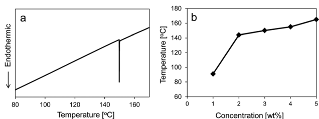
Fig. 3 (a) DSC thermograph of the ionogel of [EtMeIm][CF 3 SO 3 ] using gelator 4 (3.0 wt%). (b) Gel–sol transition temperature ( T_{\text{gel}} ) profile of the ionogel prepared with [EtMeIm][CF 3 SO 3 ] and varying concentrations of gelator 4 .
