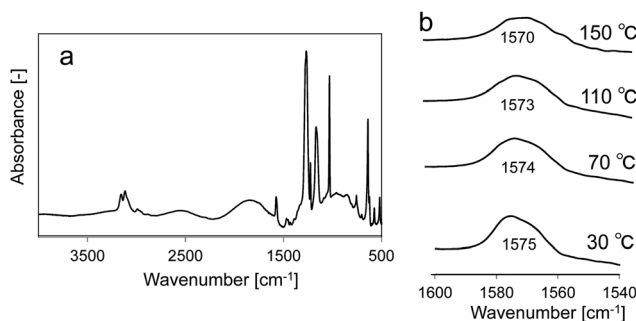
Fig. 5 (a) FTIR spectra of the ionogel prepared with [EtMeIm][CF 3 SO 3 ] and gelator 4 (0.5 wt%) at 30 °C. (b) Peak shift of the amide II band at varying temperatures from 150 to 30 °C. The associated wavelength of the peak is indicated.
