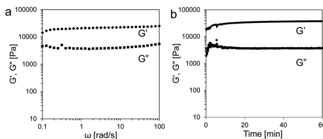
Fig. 2 Viscoelastic properties of the ionogel, prepared with [EtMeIm]–[CF 3 SO 3 ] and gelator 4 (1.0 wt%). (a) Dynamic frequency sweep at 30 °C, (b) dynamic time sweep at a frequency of 1 rad s −1 at 30 °C.
