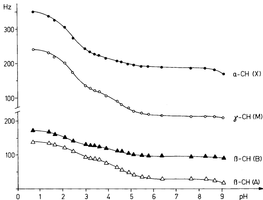
Fig. 2. ^1\text{H-NMR} -monitored titration of Gla . Solutions: 10^{-2}\text{M} Gla in aqueous NaCl ( I=0.1 ) with tetramethylammonium chloride as internal standard. The pH was adjusted with 4N NaOH and determined with a Philips Digital pH-Meter Mod. PW 9414. The spectra were measured with a Bruker HXS-360 MHz instrument with sine bell resolution enhancement [14] and Fourier transform techniques. The ordinate shows the chemical shift in Hz with respect to arbitrary, fixed points (lower Hz values indicate higher fields).
