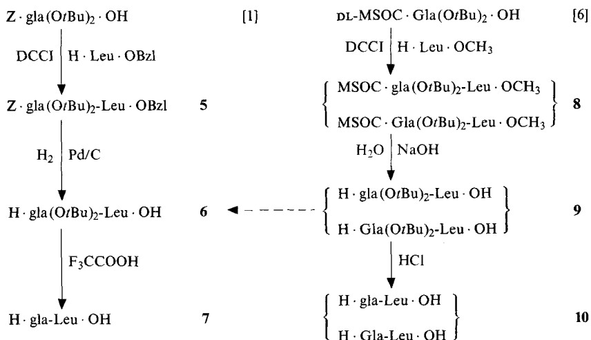
Scheme 2. Synthesis of H \cdot \text{gla-Leu} \cdot OH ( 7 ) 1)
