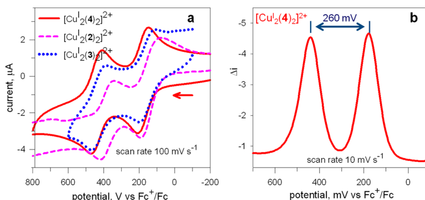
Figure 9. (a) CV profile taken at a platinum working electrode at a potential scan rate of 100 \text{ mV s}^{-1} on a MeCN solution of [\text{Cu}_2^{\text{I}}(4)_2](\text{ClO}_4)_2 , made 0.1 \text{ M} in [\text{Bu}_4\text{N}]\text{PF}_6 (solid red line); dashed lines refer to [\text{Cu}_2^{\text{I}}(2)_2]^{2+} (pink) and [\text{Cu}_2^{\text{I}}(3)_2]^{2+} (blue) complexes, investigated under the same conditions; (b) Differential Pulse Voltammetry profile taken on the same solution of [\text{Cu}_2^{\text{I}}(4)_2](\text{ClO}_4)_2 (potential scan rate 10 \text{ mV s}^{-1} ).
