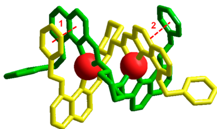
Figure 1. Crystal structure of the [\text{Cu}_2^{(RR)}]^{2+} complex. 8 A given color (whether green or yellow) has been assigned to each strand. Red dashed lines indicate the two interstrand \pi – \pi interactions between a pyridine ring of one strand and a benzyloxy subunit of the other.
