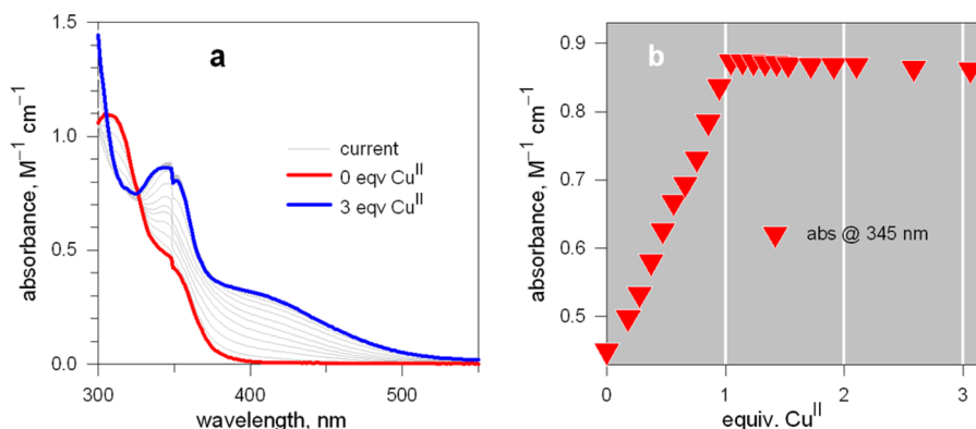
Figure 8. (a) Family of spectra recorded over the course of the titration of a 1.00 \times 10^{-4} solution of rac -5 with a 1.0 \times 10^{-2} MeCN solution of \text{Cu}^{\text{II}}(\text{CF}_3\text{SO}_3)_2 . Red line, spectrum of RR 4 prior to the titration; gray lines, current spectra; blue line, spectrum after the addition of 3 equiv of \text{Cu}^{\text{II}} ; (b) titration profile based on the absorbance at 345 nm.
