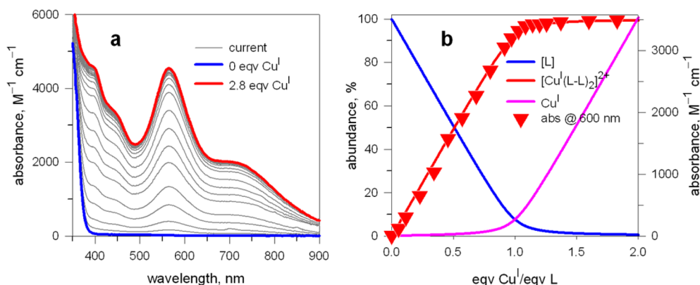
Figure 3. (a) Absorption spectra taken over the course of the titration of an MeCN solution 9.99 \times 10^{-5} M of RR 4 with a standard solution 1.03 \times 10^{-2} M in [Cu I (MeCN) 4 ] 2 ClO 4 ; (b) lines: concentration profiles (% with respect to L∩L = RR 4) of the species at the equilibrium; symbols: molar absorbance at 600 nm.
