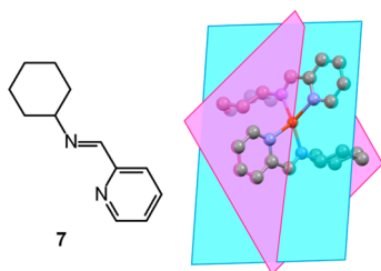
Figure 7. Crystal structure of the model complex [\text{Cu}^{\text{I}}(\mathbf{7})_2]^{+15} , showing the planes containing the five-membered chelate rings \text{Cu}\text{--N}\text{--C}\text{--C}\text{--N} . The two planes form an angle \theta = 82.5^\circ , thus indicating a moderate distortion from the tetrahedral coordination geometry (for a regular tetrahedron \theta = 90^\circ ).
