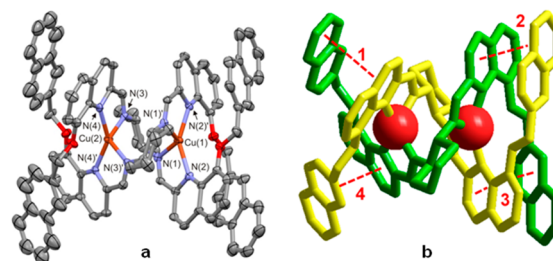
Figure 2. (a) Plot showing thermal ellipsoids of the M,M-[Cu_2^I(RR_4)_2]^{2+} helicate cationic complex (ellipsoids are drawn at the 20% probability level, atom name are reported only for the metal centers and for the bonded N atoms, symmetry code: (') = -x, 1-y, z ). (b) A tube representation of the M,M-[Cu_2^I(RR_4)_2]^{2+} helicate complex is drawn with different colors for the two symmetrically equivalent strands; the homochiral double helix shows M handedness and extensive interstrand \pi-\pi interactions (dashed lines).
