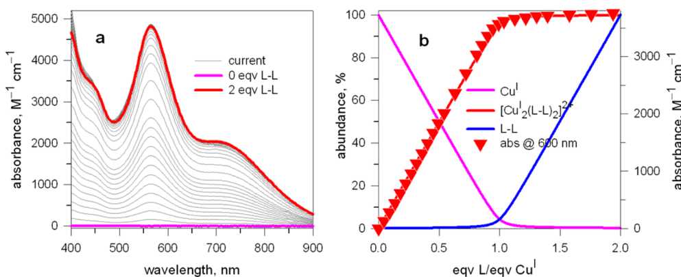
Figure 4. (a) Absorption spectra taken over the course of the titration of an MeCN solution 1.04 \times 10^{-4} M of [Cu I (MeCN) 4 ] 2 ClO 4 with a standard solution 1.03 \times 10^{-2} M in RR 4 (= L∩L); (b) lines: concentration profiles (% with respect to Cu I ) of the species at the equilibrium; symbols: molar absorbance at 600 nm.
