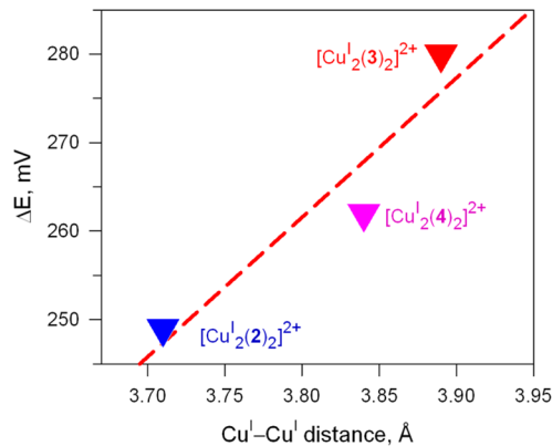
Figure 10. Plot of \Delta E ( = E_{1/2}(2) - E_{1/2}(1) in Figure 9a) vs the crystallographically determined \text{Cu}^{\text{I}}\text{--Cu}^{\text{I}} distance in [\text{Cu}_2^{\text{I}}(\text{LNL})_2](\text{ClO}_4)_2 complex salt ( \text{LNL} = 2, 7^{\text{f}}, 3, 8, 4 ).
