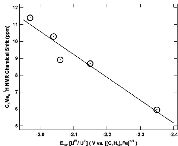
Fig. 6. Linear correlation between ^1H NMR chemical shift of C_5Me_5 protons and U^{IV}/U^{III} reduction potential for (C_5Me_5)_2U[N(SiMe_3)_2](X) ( X = F (1), Cl (2), Br (3), I (4), N_3 (5), NCO (6)).
