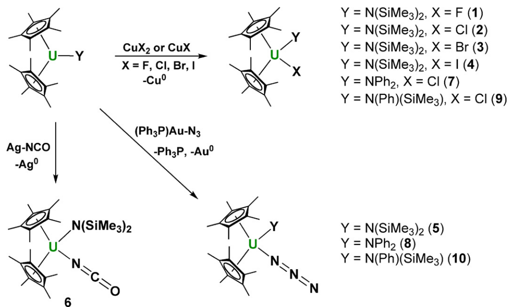
Scheme 1. Mixed-ligand U IV metallocene complexes accessed through oxidative functionalization.
