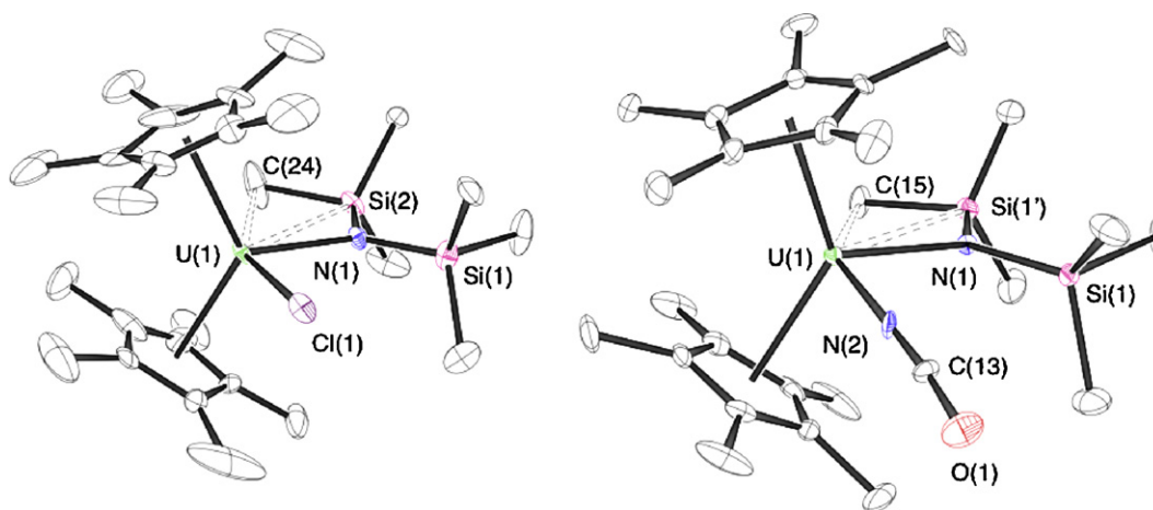
Fig. 2. Molecular structures of (C 5 Me 5 ) 2 U[N(SiMe 3 ) 2 ](Cl) ( 2 ) (left) and (C 5 Me 5 ) 2 U[N(SiMe 3 ) 2 ](NCO) ( 6 ) (right) with thermal ellipsoids projected at the 30% probability level. Hydrogen atoms have been omitted for clarity. Selected bond lengths (Å) and angles (°) for 2 : U(1)–N(1) 2.268(4), U(1)–Cl(1) 2.606(3), U(1)–C(24) 3.158, U(1)–Si(2) 3.335, Cl(1)–U(1)–N(1) 89.39(14), U(1)–N(1)–Si(1) 130.7(3), U(1)–N(1)–Si(2) 111.2(3), Si(1)–N(1)–Si(2) 118.2(3), U(1)–C(24)–Si(2) 78.2, C(24)–Si(2)–N(1) 107.3(6), N(1)–U(1)–C(24) 63.2. Selected bond lengths (Å) and angles (°) for 6 : U(1)–N(1) 2.241(11), U(1)–N(2) 2.354(16), N(2)–C(13) 1.10(2), C(13)–O(1) 1.29(2), U(1)–C(15) 3.05, U(1)–Si(1') 3.31, N(1)–U(1)–N(2) 89.2(5), U(1)–N(2)–C(13) 166.4(17), N(2)–C(13)–O(1) 174(3), U(1)–N(1)–Si(1) 128.3(6), U(1)–N(1)–Si(1') 113.2(6), Si(1)–N(1)–Si(1') 118.5(6), U(1)–C(15)–Si(1') 80.7, C(15)–Si(1')–N(1) 103.9(10), N(1)–U(1)–C(15) 62.0.
