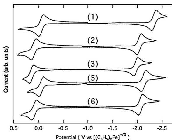
Fig. 5. Cyclic voltammograms obtained at 200 mV/s scan rate for \sim 2 –5 mM solutions of (C_5Me_5)_2U[N(SiMe_3)_2](X) ( X = F ( 1 ), Cl ( 2 ), Br ( 3 ), N_3 ( 5 ), and NCO ( 6 )) in \sim 0.1 M [Pr_4N][B(3,5-(CF_3)_2C_6H_3)_4]/THF at a Pt disk electrode.
