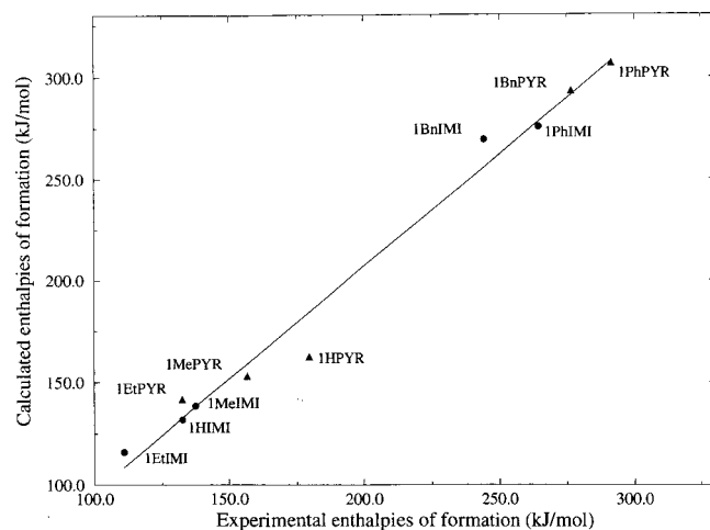
Figure 2. Linear correlation between calculated and experimental enthalpies of formation [ \Delta_f H_m^\circ(\text{cal.}) = (1.10 \pm 0.05)\Delta_f H_m^\circ(\text{exp.}) - (13.5 \pm 10.2) \text{ kJ mol}^{-1} , R^2 = 0.984 ] for the N-substituted imidazoles (●) and N-substituted pyrazoles (▲). For imidazoles, the calculated values were obtained through the use of the quasiisodesmic reactions 9–13, while for pyrazoles, the quasiisodesmic reactions 14–18 were used.
