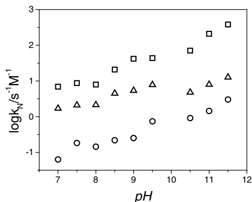
Figure 3. Variation of \log k_{\text{N}} as a function of pH for the reactions of PAA with NPC (O), DNPC (Δ) and TNPC (□) in aqueous solution at 25.0 °C and an ionic strength of 0.1 M (KCl)
