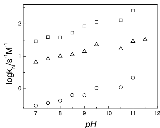
Figure 2. Variation of \log k_{\text{N}} as a function of pH for the reactions of PAA with NPA (O), DNPA (Δ) and TNPA (□) in aqueous solution at 25.0 °C and an ionic strength of 0.1 M (KCl)
