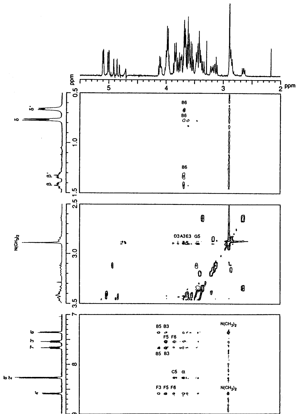
Figure 6. 500 MHz ROESY spectrum of 1 in D 2 O at 25 °C with mixing time of 300 ms, indicating the cross peaks between the protons of the dansyl-L-leucine moiety and the protons of the \beta -CD moiety.
