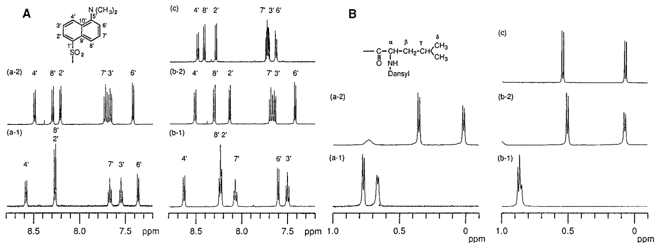
Figure 5. 500 MHz ^1\text{H} NMR spectra of 1 (a-1) alone, (a-2) in the presence of 1-adamantanol, 2 (b-1) alone, (b-2) in the presence of 1-adamantanol, and (c) 7 in \text{D}_2\text{O} at 25 ^\circ\text{C} in the region of (A) aromatic protons and (B) \delta protons of leucine: [\mathbf{1}] = [\mathbf{2}] = [\mathbf{7}] = [\text{1-adamantanol}] = 1 \times 10^{-3} \text{ M} .
