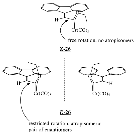
Figure 2. Stereoisomers of 26 at -40 °C.
