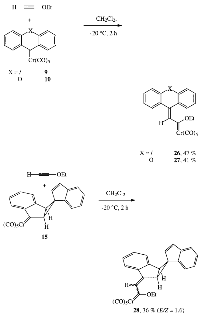
Scheme 6. Ynol Ether Insertion Reactions of Carbene Complexes 9, 10, and 15
