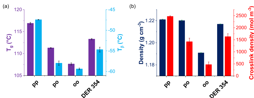
Figure 4. Physical properties of networks produced using MXDA as the amine monomer and para-para - (pp), para-ortho - (po), and ortho-ortho - (oo)-DGEGBF or Dow Epoxy Resin 354 (DER 354) as the epoxide monomer. (a) Glass transition temperature ( T_g ), the \beta -transition temperature ( T_\beta ) as determined by DMA and (b) crosslink density as determined by DMA (calculated from eq 2—see Experimental Section) and density as determined by helium pycnometry. Error bars show standard error for three samples for T_g and crosslink density, standard error for two samples for T_\beta and standard deviation of ten measurements of a single sample for density.
