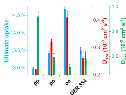
Figure 6. Chemical performance in methanol of networks produced using MXDA as the amine monomer and para-para - (pp), para-ortho - (po), and ortho-ortho - (oo)-DGEGBF or Dow Epoxy Resin 354 (DER 354) as the epoxide monomer. Shown are the ultimate uptake (by original mass) of each network and the diffusion coefficients of sorption ( D_{sor} ) and desorption ( D_{des} ) at 40 °C. Error bars show standard error of the three samples.
