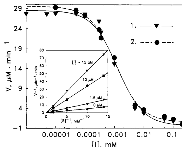
Figure 1. Inhibition of human skin fibroblast collagenase by (EtO)(OK)P(O)-Ile-Trp-NHCH 3 (68) using the thiol ester substrate (▼) at pH 6.5 and the amide substrate assay (●) at pH 7.5. Inset: a Lineweaver-Burk plot of the same inhibitor 68 using the thiol ester substrate.
