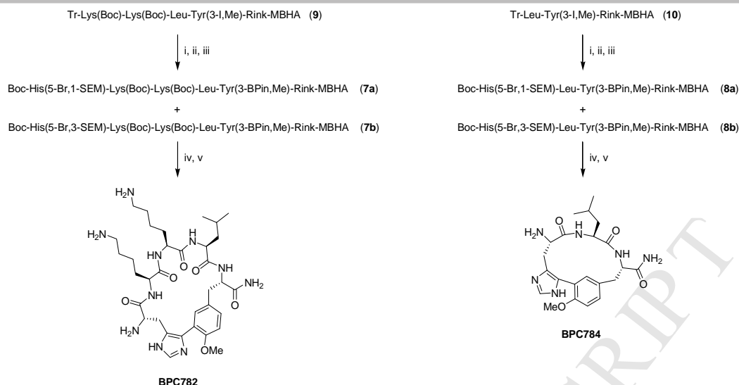
Scheme 2. Solid-phase synthesis of biaryl cyclic peptides BPC782 and BPC784 . Reagents and conditions: (i) B_2Pin_2 , PdCl_2(dppf) , dppf , KOAc , DMSO , 80\text{ }^\circ\text{C} , 8 h. (ii) TFA/H_2O/CH_2Cl_2 (0.2:1:98.8) (2×1 + 2×20 min). (iii) Boc\text{-His(5-Br,1-SEM)-OH} ( 5a ) and Boc\text{-His(5-Br,3-SEM)-OH} ( 5b ), DIPCDI , Oxyma , DMF , 3 h. (iv) Pd_2(dba)_3 , KF , SPhos , DME/EtOH/H_2O , MW , 140\text{ }^\circ\text{C} , 30 min. (v) TFA/H_2O/TIS (95:2.5:2.5), 3 h, stirring.
