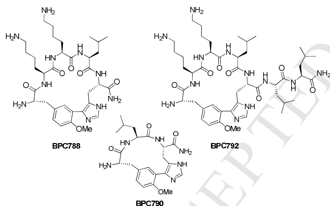
Fig.3. Structure of biaryl cyclic peptides containing a His at the C-terminus.
