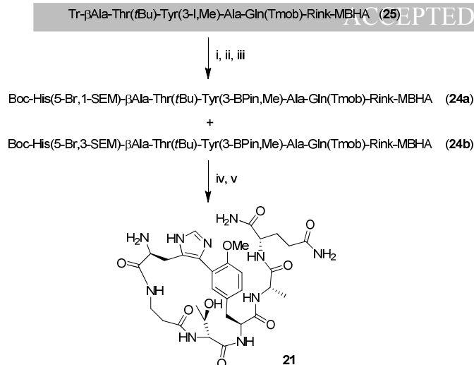
Scheme 6. Solid-phase synthesis of the biaryl cyclic peptide 21 . Reagents and conditions: (i) B_2Pin_2 , PdCl_2(dppf) , dppf, KOAc, DMSO, 80 °C., 8 h. (ii) TFA/H 2 O/CH 2 Cl 2 (0.2:1:98.8), (2×1 + 2×20 min). (iii) Boc-His(5-Br,1-SEM)-OH ( 5a ) and Boc-His(5-Br,3-SEM)-OH ( 5b ), DIPCDI, Oxyma, DMF, 3 h. (iv) Pd_2(dba)_3 , SPhos, KF, DME/EtOH/H 2 O, MW, 140 °C, 30 min. (v) TFA/H 2 O/TIS (95:2.5:2.5), 3 h, stirring.
