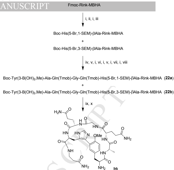
Scheme 5. Solid-phase synthesis of the biaryl cyclic peptide 20 . Reagents and conditions: (i) Piperidine/DMF (3:7) (2 + 10 min). (ii) Fmoc- \beta Ala-OH, DIPCPI, Oxyma, DMF, 1 h. (iii) Boc-His(5-Br,1-SEM)-OH ( 5a ) and Boc-His(5-Br,3-SEM)-OH ( 5b ), COMU, Oxyma, DIEA, DMF, overnight. (iv) TMSOTf, 2,6-lutidine, CH 2 Cl 2 (10×30 min). (v) Fmoc-Gln(Tmob)-OH, DIPCPI, Oxyma, DMF, 1 h. (vi) Fmoc-Gly-OH, DIPCPI, Oxyma, DMF, 1 h. (vii) Fmoc-Ala-OH, DIPCPI, Oxyma, DMF, 1 h. (viii) Boc-Tyr(3-B(OH) 2 ,Me)-OH, DIPCPI, Oxyma, DMF, 3 h. (ix) Pd 2 (dba) 3 , KF, SPhos, DME/EtOH/H 2 O, MW, 140 °C, 30 min. (x) TFA/H 2 O/TIS (95:2.5:2.5), 3 h, stirring.
