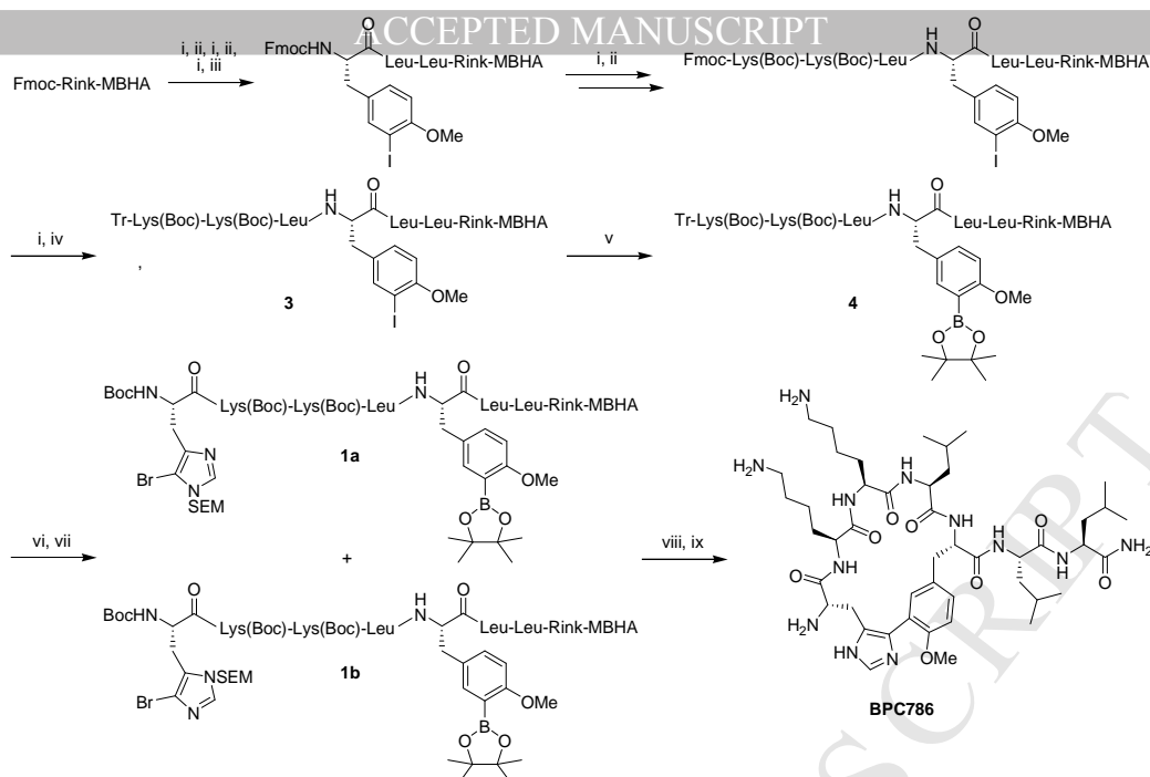
Scheme 1. Solid-phase synthesis of the biaryl cyclic peptide BPC786 . Reagents and conditions: (i) Piperidine/DMF (3:7) (2 + 10 min). (ii) Fmoc-Leu-OH or Fmoc-Lys(Boc)-OH, DIPCDI, Oxyma, DMF, 1 h. (iii) Fmoc-Tyr(3-I,Me)-OH ( 2 ), COMU, Oxyma, DIEA, DMF, overnight. (iv) TrCl, DIEA, DMF, 4 h. (v) B_2Pin_2 , PdCl_2(dppf) , dppf, KOAc, DMSO, 80 °C, 8 h. (vi) TFA/ H_2O/CH_2Cl_2 . (0.2:1:98.8) (2×1 + 2×20 min). (vii) Boc-His(5-Br,1-SEM)-OH ( 5a ) and Boc-His(5-Br,3-SEM)-OH ( 5b ), DIPCDI, Oxyma, DMF, 3 h. (viii) Pd_2(dba)_3 , KF, SPhos or P(o\text{-tolyl})_3 , DME/ EtOH/H_2O , MW, 140 °C, 30 min. (ix) TFA/ H_2O/TIS (95:2.5:2.5), 3 h, stirring.
