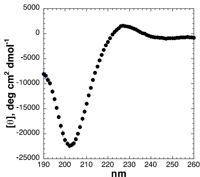
Figure 3. CD spectrum of Ac-GPP(Hse(C 4 F 9 ))PPGY-NH 2 in the model peptide context previously employed(100, 105, 126, 141) to determine polyproline II helix propensities of guest amino acids at the indicated position of substitution. Experiments were conducted in 5 mM phosphate buffer with 25 mM KF at pH 7.4 at 25 °C. Extent of PPII is indicated by [\theta]_{228} = 1500 \pm 190 \text{ deg cm}^2 \text{ dmol}^{-1} . The ^3J_{\alpha\text{N}} for Hse(C 4 F 9 ) is 7.7 Hz, compared to ^3J_{\alpha\text{N}} = 7.2 \text{ Hz} for Met in this position in this peptide context.
