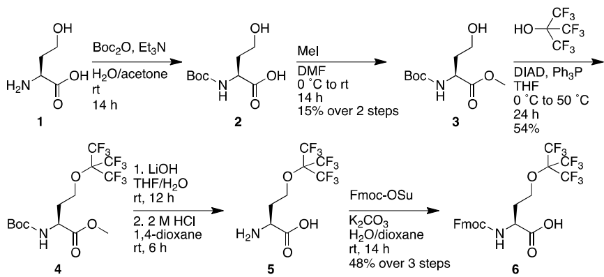
Scheme 1. Synthesis of Fmoc-perfluoro- tert -butyl homoserine ( 6 ) from homoserine ( 1 ). 2 is also commercially available.
