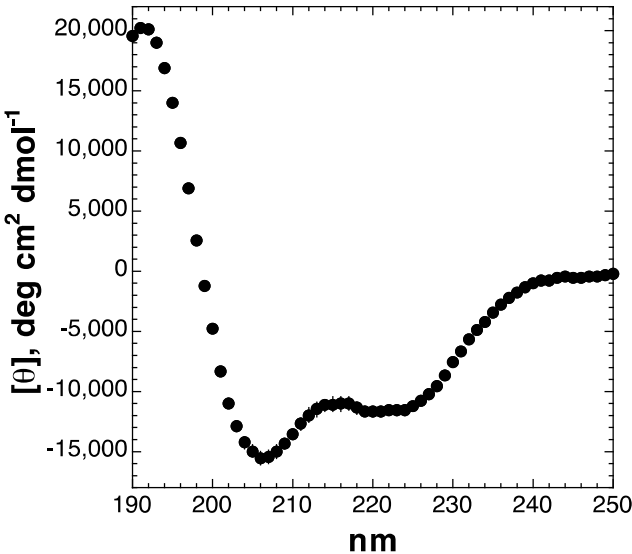
Figure 2. CD spectrum of Ac-(Hse(C 4 F 9 ))KAAA KAAA KAAGY-NH 2 in the Baldwin-type α-helical model peptide previously employed(100, 106) to determine the structural effects of serine and threonine phosphorylation and O-GlcNAcylation on α-helix stability. Experiments were conducted in 5 mM phosphate buffer with 25 mM KF at pH 7.4 at 0.5 °C. Extent of α-helical structure is indicated by [\theta]_{222} = -11510 \pm 400 \text{ deg cm}^2 \text{ dmol}^{-1} , [\theta]_{222}/[\theta]_{208} = 0.77 , corresponding to 36% α-helix.(112, 113) Error bars are shown and indicate standard error. The ^3J_{\alpha\text{N}} (Figure S5), which correlates with the \phi torsion angle (smaller value = more compact \phi ),(107) is 6.4 Hz for Hse(C 4 F 9 ) in this peptide, similar to that of Thr (6.2 Hz) at this position in this peptide context, and greater than that of the more α-helical Ser (5.1 Hz) at this position in this peptide context.
