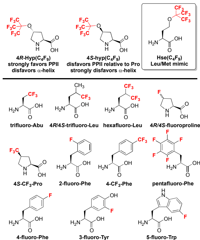
Figure 1. Top: perfluoro- tert -butyl amino acids; bottom: selected aliphatic and aromatic fluorinated amino acids used for 19 F NMR-based detection.
