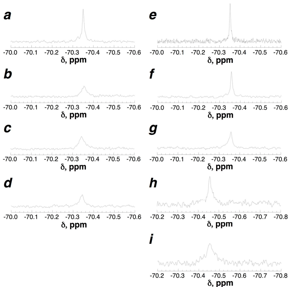
Figure 6. ^{19}\text{F} NMR spectroscopy of the peptide Leu12Hse(C 4 F 9 ). Experiments were conducted with 5 \mu\text{M} peptide in 1 \times PBS (pH 7.4), 0.1 mM DTT, 20 \mu\text{M} estradiol (except g), and 10% D 2 O. (a-e) The peptide Leu12Hse(C 4 F 9 ) with (a) no added protein; (b) 5 \mu\text{M} ER \alpha LBD; (c) 15 \mu\text{M} ER \alpha LBD; (d) 30 \mu\text{M} ER \alpha LBD; and (e) 30 \mu\text{M} bovine gamma globulin. (f) 5 \mu\text{M} peptide Leu12Hse(C 4 F 9 ) with 15 \mu\text{M} ER \alpha LBD and 20 \mu\text{M} NRBox II. (g) 5 \mu\text{M} peptide Leu12Hse(C 4 F 9 ) with 15 \mu\text{M} ER \alpha LBD and 50 \mu\text{M} 4-hydroxytamoxifen (OHT), without added estradiol. (h-i) The peptide Leu12Hse(C 4 F 9 ) (h) with 200 \mu\text{L} HeLa cell lysates and (i) with 200
