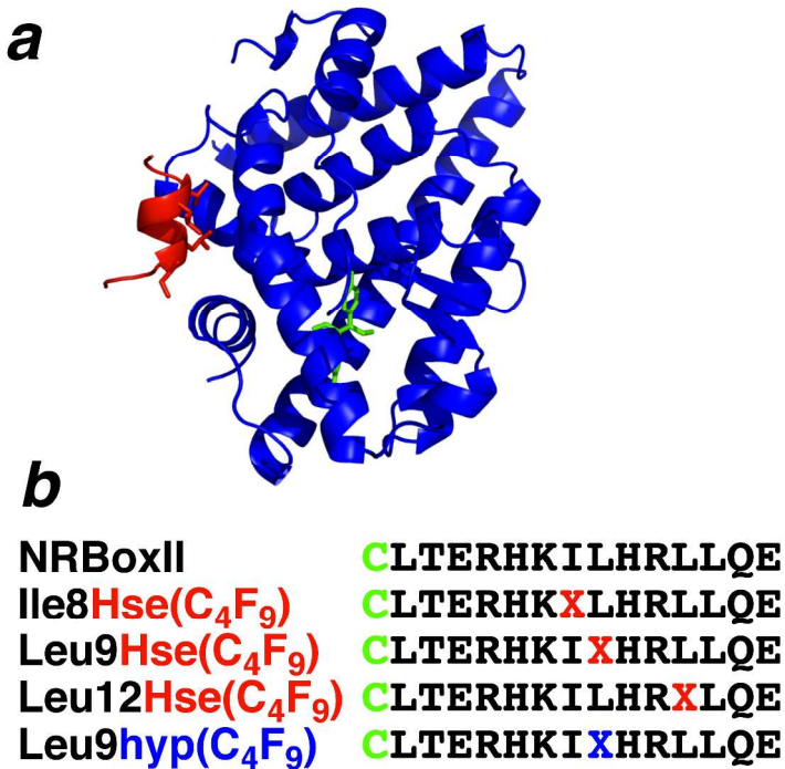
Figure 4. (a) X-ray crystal structure (pdb 3erd)(22) of the estrogen receptor- \alpha ligand-binding domain (ER \alpha LBD, residues 305-550, blue) bound to the estrogen mimic diethylstilbestrol (green) and the GRIP1 NRBoxII co-activator peptide (HKILHRL L QDS, red). Coactivator peptides bind to the ligand-bound estrogen receptor via one face of an \alpha -helix containing the LXXLL short linear motif (side chains shown). (b) Peptide designs for the incorporation of perfluoro- tert -butyl amino acids into estrogen receptor coactivator peptides. X indicates the site of modification with a perfluoro- tert -butyl amino acid, with either Hse(C 4 F 9 ) (red) or 4 S -hyp(C 4 F 9 ) (blue) substitution at the indicated residue. All peptides for fluorescence polarization experiments were labeled with 5-iodoacetamidofluorescein on Cys (green). Peptides used in NMR spectroscopy experiments lacked the N-terminal Cys. All peptides were acetylated on the N-terminus and contain C-terminal amides. Details of the synthesis and characterization of peptides are in the Supporting Information.
