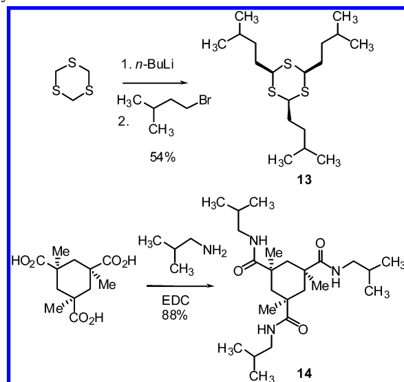
Scheme 4. Synthesis of Trithiane- and Cyclohexane-Core CBIs
