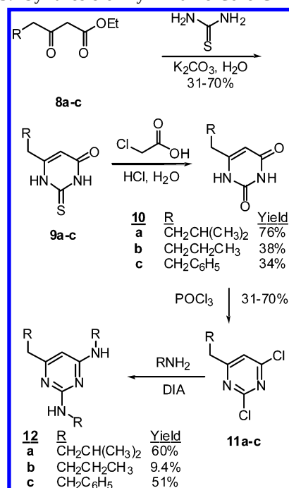
Scheme 4. Synthesis of Trithiane- and Cyclohexane-Core CBIs
