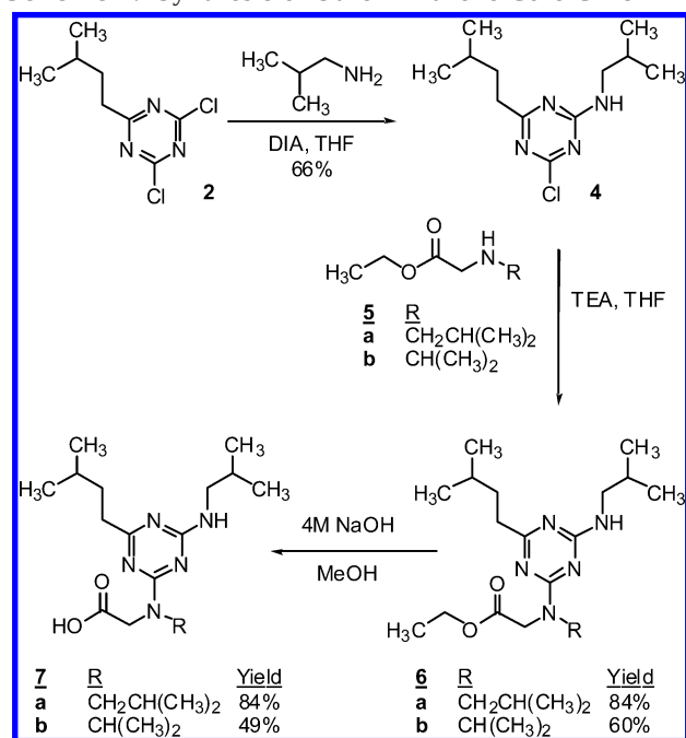
Scheme 2. Synthesis of Other Triazene-Core CBIs
