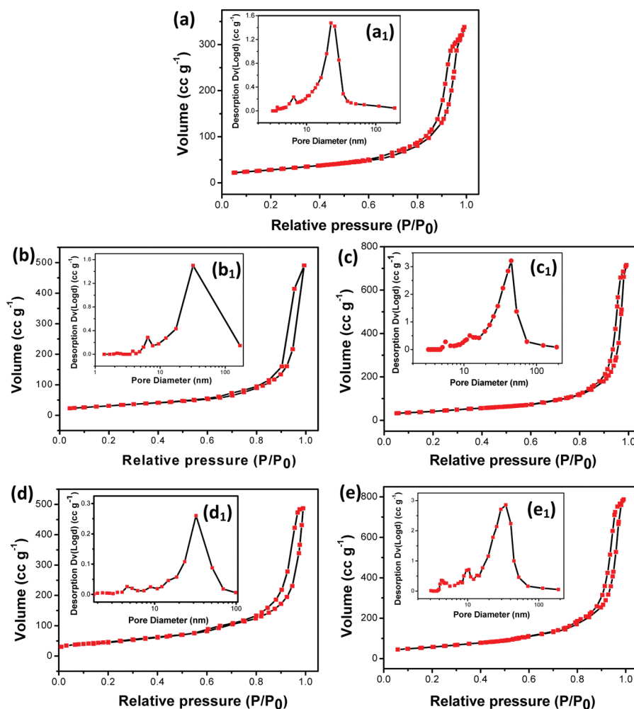
Figure 3. N_2 adsorption–desorption isotherms (a–e) and pore diameter distribution ( a_1 – e_1 ) of the hydrothermally synthesized (Ni_{1-x}Mg_x)_3Si_2O_5(OH)_4 solid-solution NTs, with molar ratios of Mg^{2+}:Ni^{2+} = 0:2.0 (a and a_1 ), 0.5:1.5 (b and b_1 ), 1.0:1.0 (c and c_1 ), 1.5:0.5 (d and d_1 ), and 2.0:0 (e and e_1 ).
