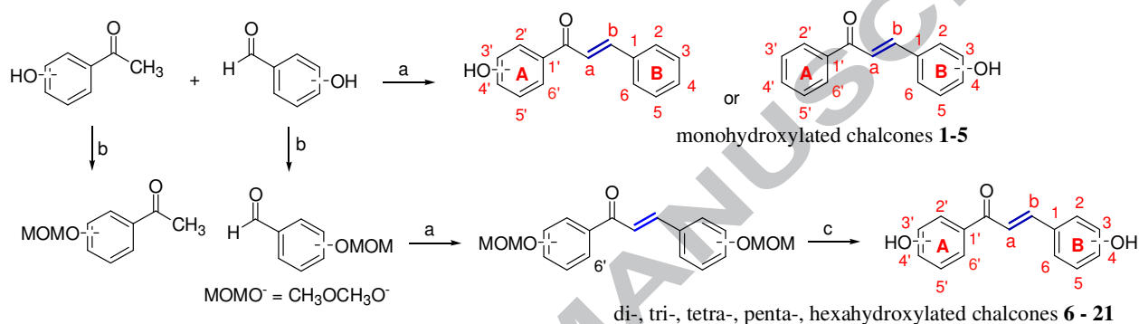
Figure 2. Synthesis of chalcones. Reaction conditions: a) 20% KOH, EtOH, room temperature, 24 – 72 h; b) \text{CH}_3\text{OCH}_2\text{Cl} , \text{K}_2\text{CO}_3 , acetone, reflux, 4 h; c) 10% HCl, EtOH, reflux, 15 min.
