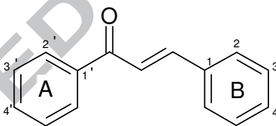
The chalcone scaffold.
