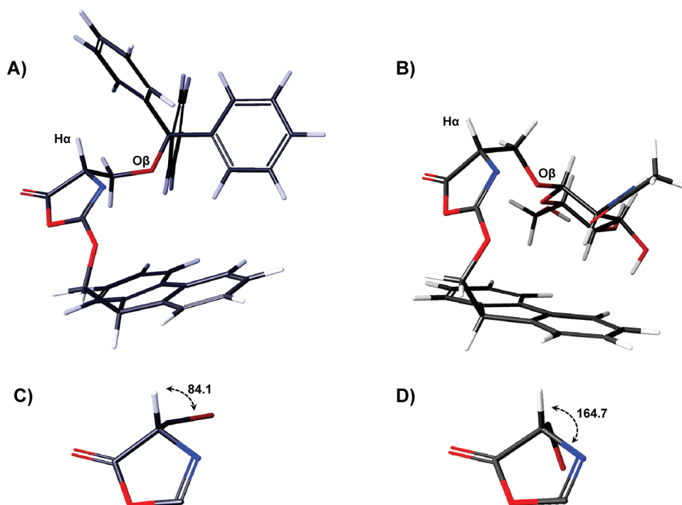
Figure 6. Low-energy models of the oxazolone intermediates derived from (A) Fmoc-Ser(Trt)-OH and (B) Fmoc-Ser(Ac 3 GlcNAcβ)-OH ( 13 ) generated from the Conformational Search utility in MacroModel 2011. Panels (C) and (D) are expansions of the oxazolone ring with the H \alpha -C \alpha -C \beta -O \beta dihedral angle value labeled.
