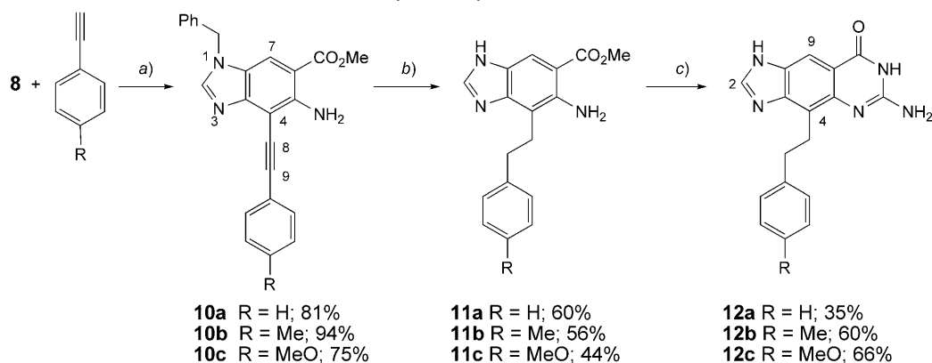
Scheme 2. Synthesis of Inhibitors 12a–12c
