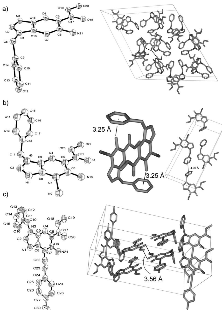
Fig. 4. a) X-Ray crystal structure of 7b (left) with unit cell (right). b) X-Ray crystal structure of 8 (left) with the N -H/ \pi interactions (middle), and the unit cell (right). c) X-Ray crystal structure of 10b (left) with the unit cell (right). Arbitrary numbering. Atomic displacement parameters in the ORTEP plots obtained at 293 K are drawn at the 50% probability level.
