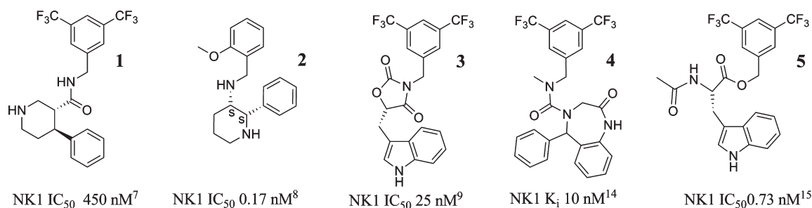
Figure 1. Structures of reported peptidomimetic NK1R antagonists.
