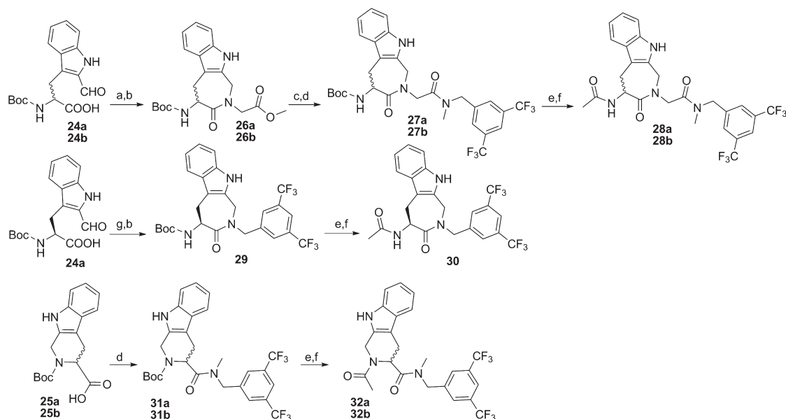
Scheme 3. Synthesis of Aia and Tcc Analogues 28a/b , 30 , and 32a/b a
