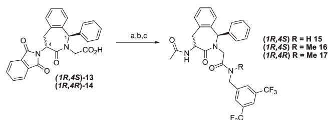
Scheme 1. Synthesis of 1-Phenyl Aba Analogues 15 – 17 a
