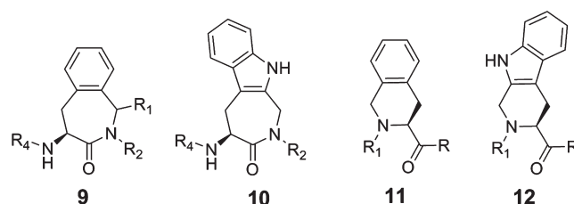
Figure 3. General structures of the 9 (Aba), 10 (Aia), 11 (Tic), and 12 (Tcc) scaffolds.
