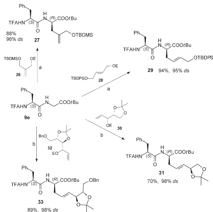
Scheme 7. Regioselective introduction of several functionalized side chains. Reaction conditions: a) allylic substrate (0.7 equiv), [\text{allylPdCl}_2] (1.4 mol%), \text{PPh}_3 (6.3 mol%), LHMDS (3.5 equiv), \text{ZnCl}_2 (1.2 equiv), THF, -78 \rightarrow -55^\circ\text{C} ; b) the same as (a), but warming to 0^\circ\text{C} was required. TBDMS = tert -butyldimethylsilyl, TBDPS = tert -butyldiphenylsilyl ether.
