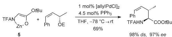
Scheme 2. Isomerization-free allylation of chelated glycine ester 5 . TFA = trifluoroacetyl.
